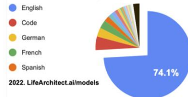
PaLM - 122 languages
