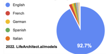
GPT-3 - 90 languages
