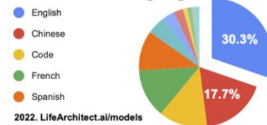
BLOOM - 46 languages
